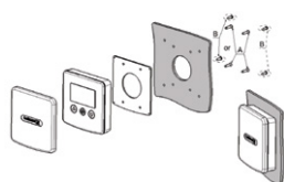
WALL MOUNTING
