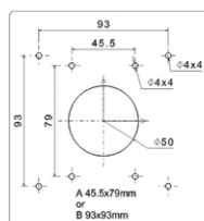
WALL MOUNTING
