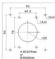
WALL MOUNTING
