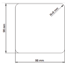
PANEL MOUNTING
