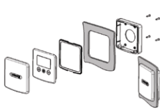
PANEL MOUNTING
